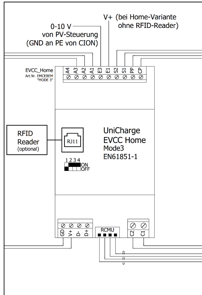
Figure 35 Charge controller schematic 0-10 V interface
