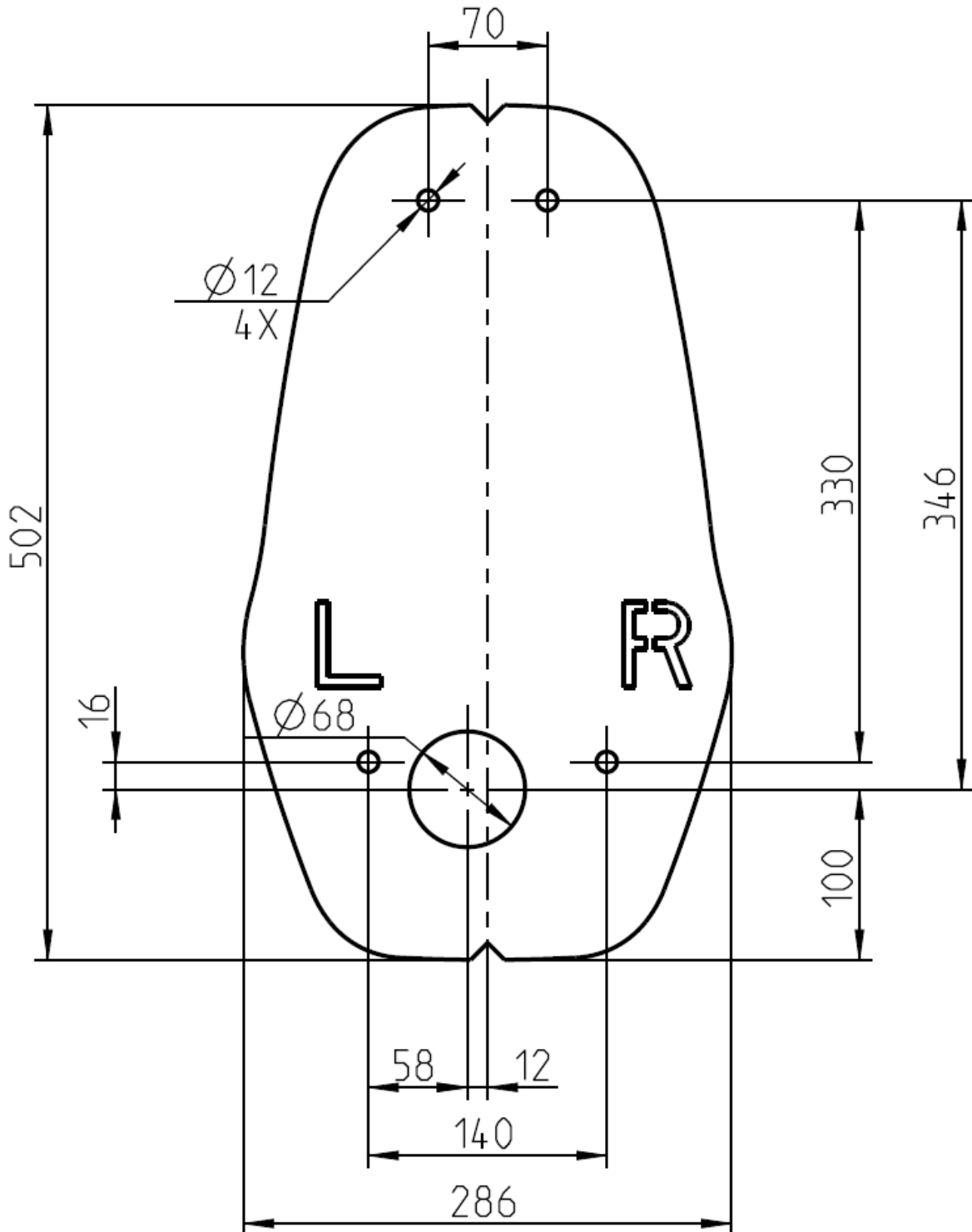
Figure 40 Drill template
