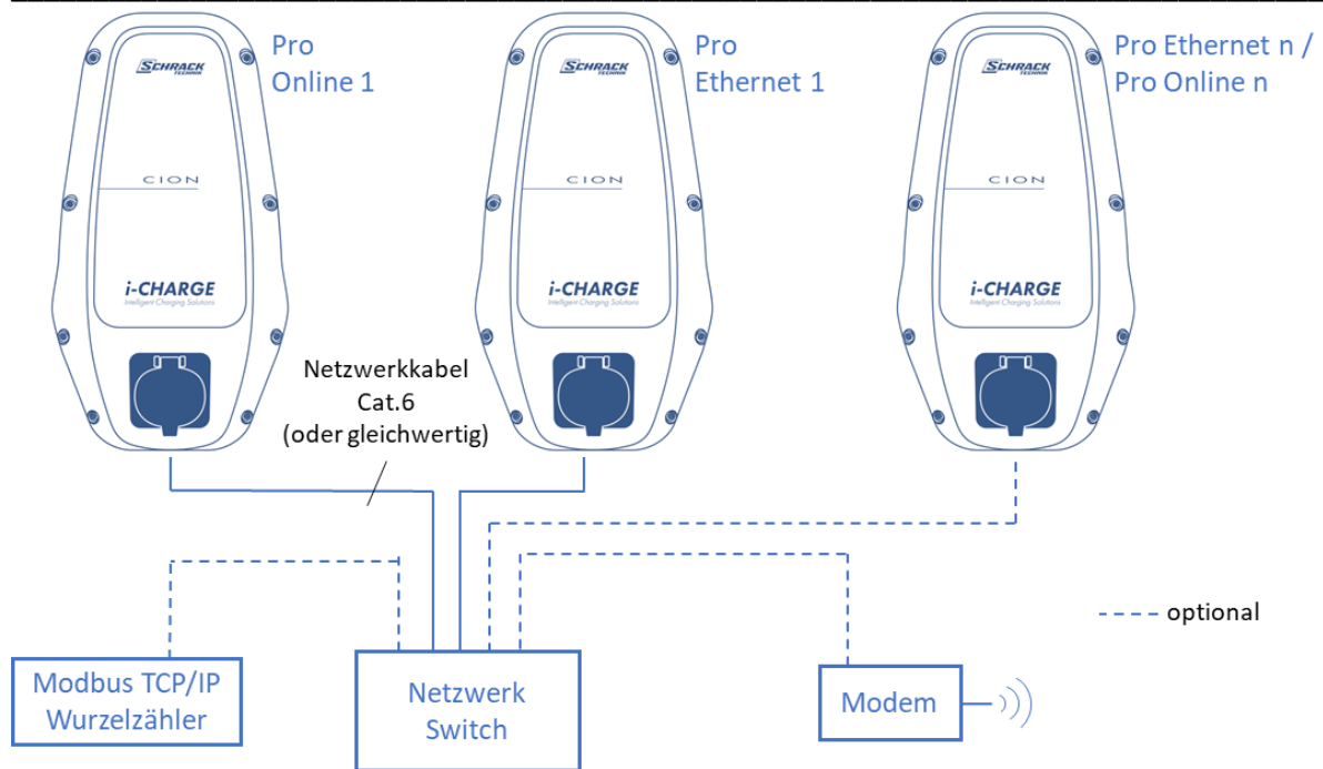
Figure 37 CION Pro wiring schematic
