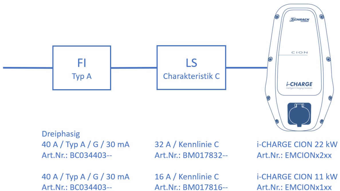
Figure 38 Back-up fuse schematic
