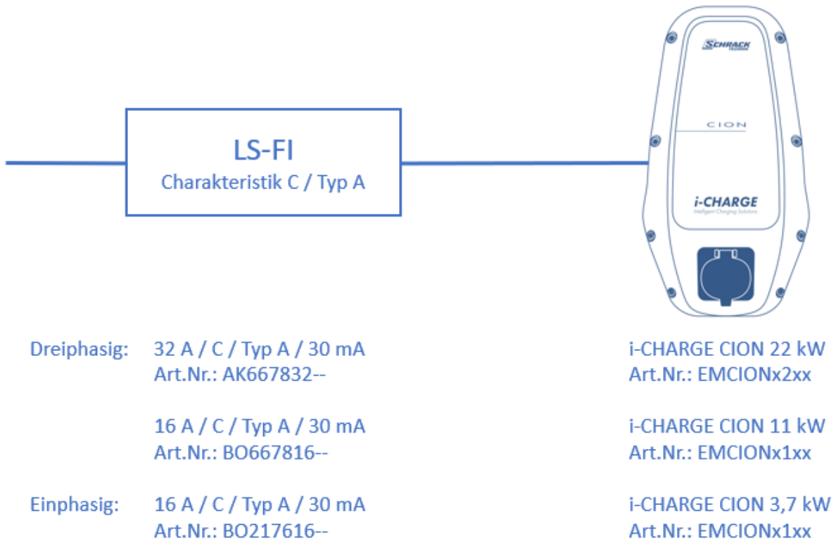
Figure 39 Back-up fuse schematic
